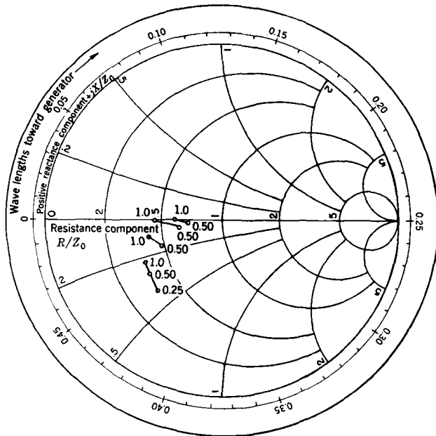
FIG. 2-23.—Change of r-f impedance with rectified crystal current. The numbers indicate rectified current in milliamperes, \lambda_{r-f} = 9.8 cm.
