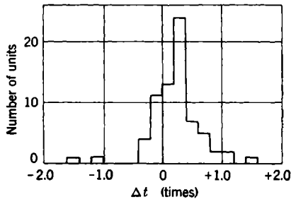
FIG. 6-6.—Difference in noise temperature of 1N26 rectifiers. \Delta t = t_1 - t_2 , where t_1 is the noise temperature for \lambda_{r-f} = 3.2 cm, \nu_{i-f} = 30 Mc/sec and t_2 is the noise temperature for \lambda_{r-f} = 1.25 cm, \nu_{i-f} = 60 Mc/sec. Data are for the same units plotted in Fig. 6-5.
