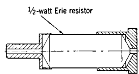
FIG. 9-28.—Resistor cartridge.
