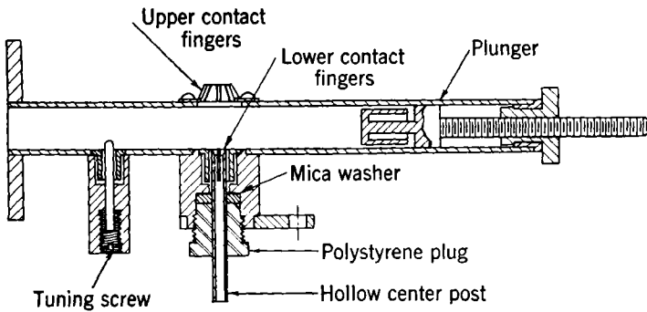
FIG. 9-5.—Crystal holder.
