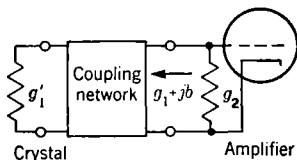
FIG. 7-12.—Block diagram of input coupling network for noise-temperature measurements.
