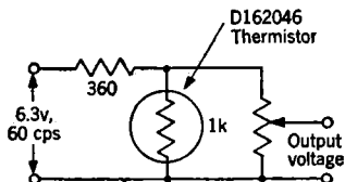
FIG. 9-7.—Regulator for modulator voltage.
