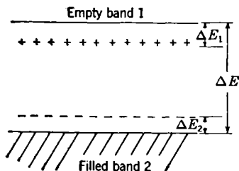
FIG. 3-2.—Band structure of an extrinsic semiconductor showing positions of donator levels (+) and acceptor levels (-).
