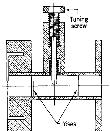
FIG. 9-25.—R-f filter.
