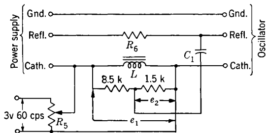
FIG. 9-6.—Modulation circuit.
