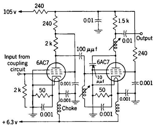
FIG. 9-29.—Preamplifier circuit.
