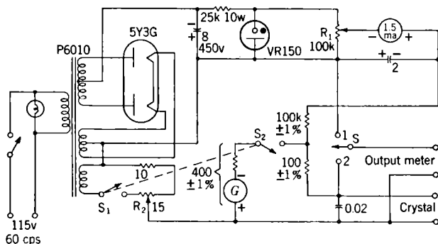
FIG. 9-16.—Output circuit.
