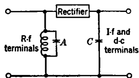
FIG. 5-1.—Transformation from a two-terminal to a four-terminal mixer.
