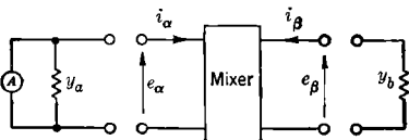
FIG. 5-6.—Mixer-terminal conditions for arbitrary image load considered as part of the mixer.
