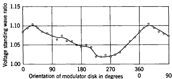
FIG. 9-21.—Standing-wave ratio of mechanical modulator.
