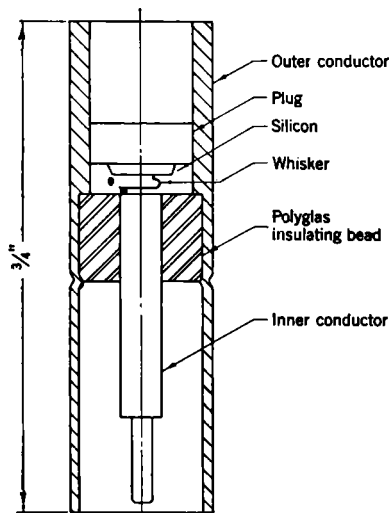
FIG. 2-4.—Coaxial cartridge.
