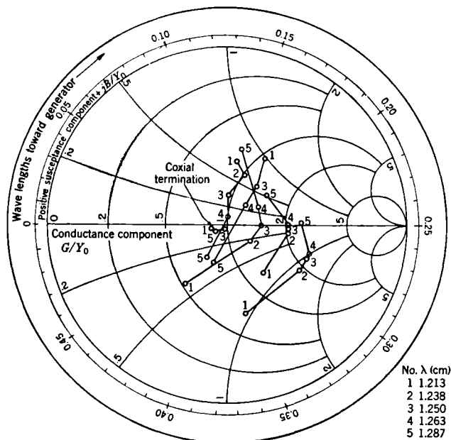
FIG. 2-24.—R-f admittance as a function of frequency. The points are numbered in order of increasing wavelength.
