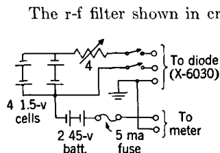
FIG. 9-26.—Diode power supply.
