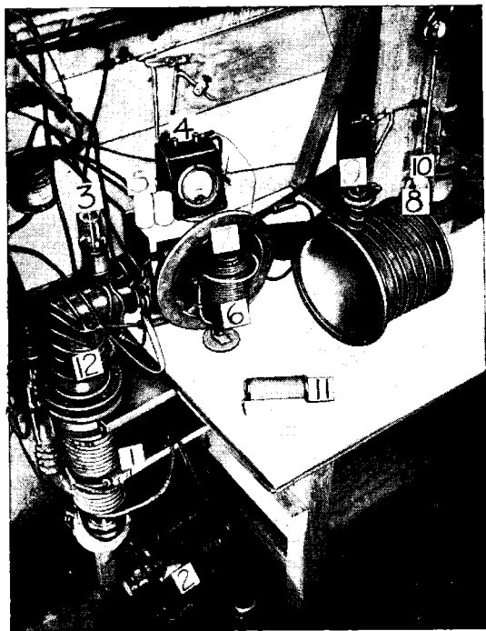
FIG. 10-2.—Vacuum furnace for melting silicon.
