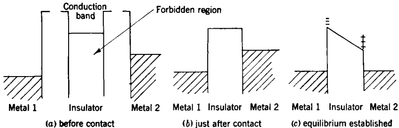
FIG. 4-1.—Formation of a rectifying barrier between two metals of different work function.
