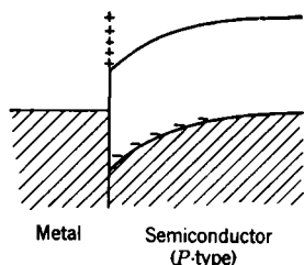
FIG. 4-4.—Barrier between a metal and a p -type semiconductor.
