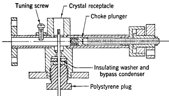
FIG. 9-15.—Crystal holder for the 1-cm test equipment.
