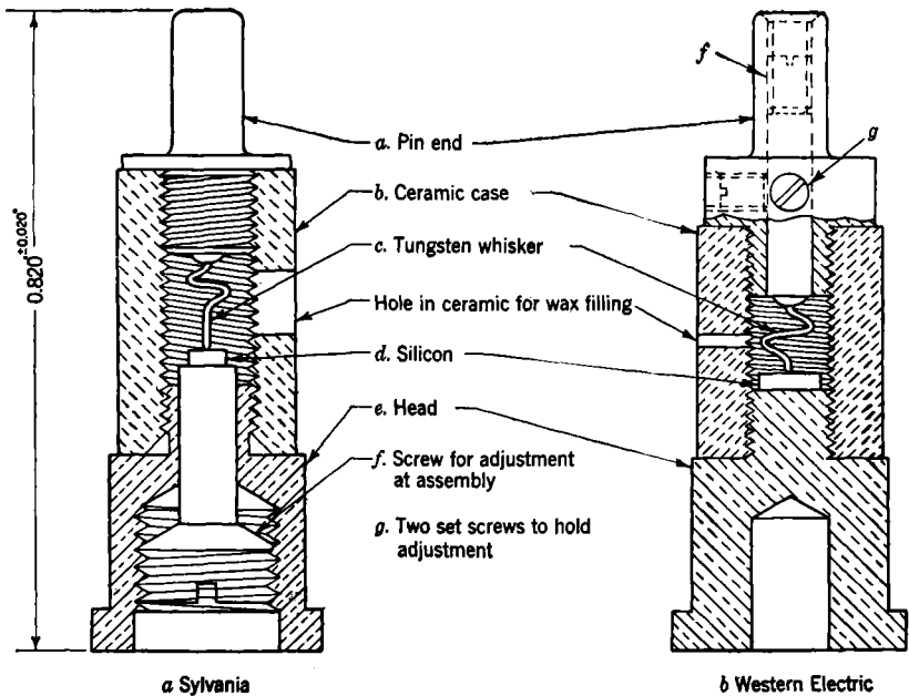
FIG. 2-2.—Ceramic cartridges.
