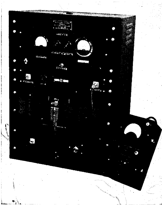
FIG. 9-10.—The conversion-loss set for the 10-cm band.
