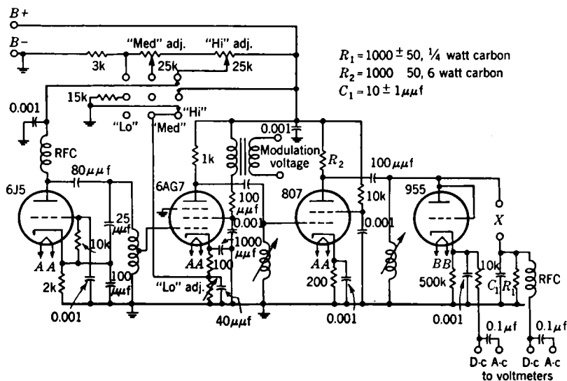
FIG. 12-18.—Type B test set for measuring over-all performance of crystal second detectors for an intermediate frequency of 30 Mc/sec.
