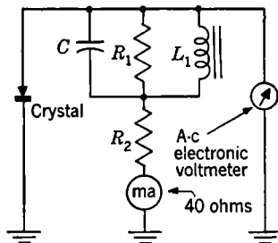
FIG. 9-8.—Crystal output circuit.
