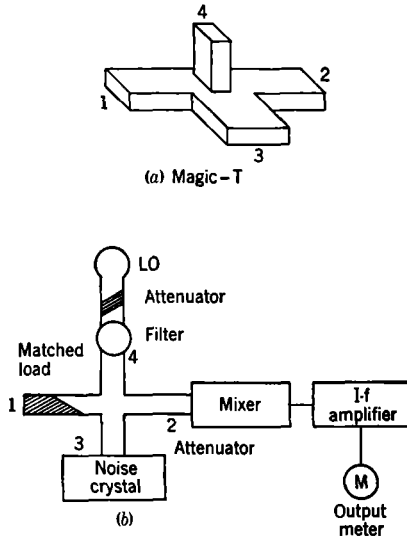
FIG. 6-11.—Apparatus for measuring the r-f noise temperature of a crystal rectifier.
