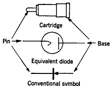
FIG. 2-3.—Cartridge polarity.
