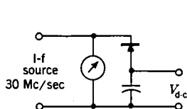
FIG. 12-14(a).—Circuit for the measurement of peak inverse voltage at 30 Mc/sec.
