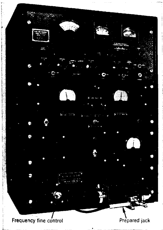
FIG. 9-31.—Noise-measuring set for the 10-cm band.
