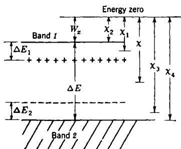
FIG. 3-3.—Band structure of a semiconductor showing work functions ( \chi, \chi_1, \chi_2, \dots ) that apply in various special cases.
