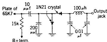
FIG. 9-30.—Output-meter circuit.
