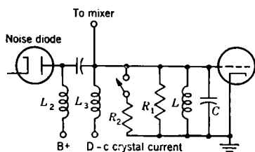
FIG. 7-15.—Input circuit for the laboratory measurement of mixer crystal properties.
